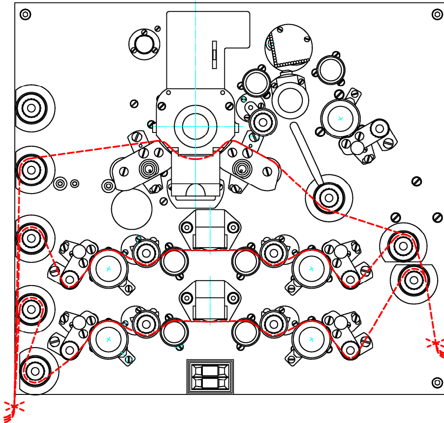
ST901-ST1901: picture w/o sound with SEPMAG
