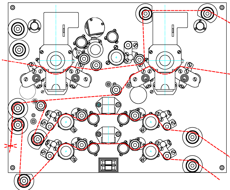
ST921: picture L with COMOPT / COMMAG / SEPMAG
