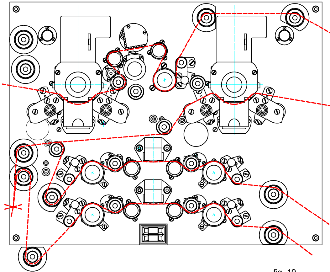
ST921: picture L with COMOPT / COMMAG / SEPMAG
