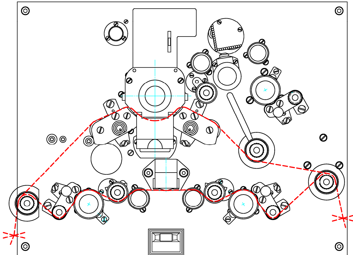
ST601-ST1601: picture w/o sound with SEPMAG
