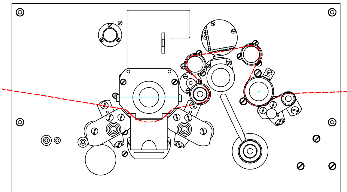
ST1201: picture with optical sound COMOPT or COMMAG
