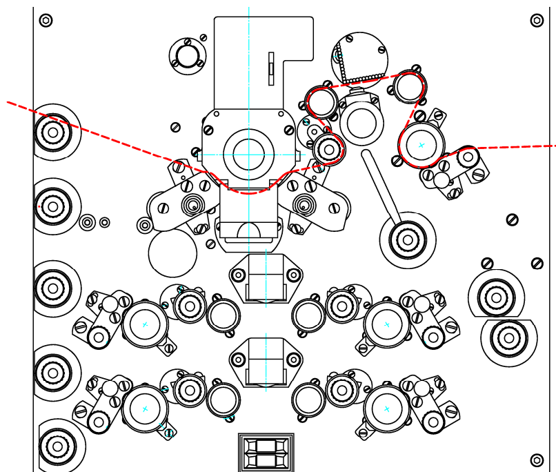
ST901-ST1901: picture with COMOPT or COMMAG fig. 17
